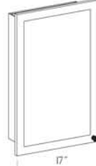
Vanity Wall Recess (VWR) Available sizes: Width: 14 1/4 Depth: 3 1/4 Height: 18, 24
