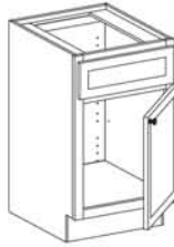
Vanity Sink Base (VSB) Available sizes: Width: 18, 21 Depth: 16, 18, 21 Height: 33 1/2
