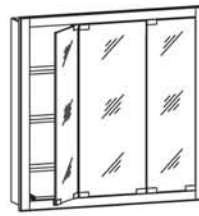
TriView Mirror (TV-PC) Polished Chrome, (TV-PB) Polished Brass or (TV-SN) Satin Nickel or (TV-VB) Venetian Bronze Available sizes: Width: 24, 30, 36, 48 Depth: 4 1/4 Height: 30
