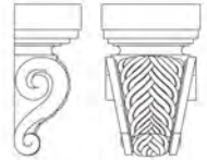
Braid Corbel (BRC) Available sizes: Width: 2 1/4, 5 1/2, 5 3/4 Depth: 2 1/2, 3, 3 3/4, 4 Height: 6, 9, 13, 13 1/2
