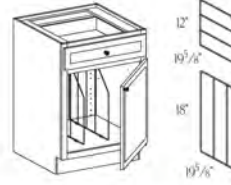
Wire Tray Dividers (WTDK) Available sizes: Height: 12, 18 Depth: 19 1/4
